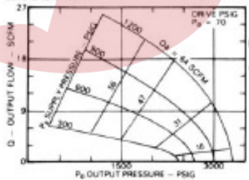
MODEL AAD — 30 Double Acting — Single Stage
