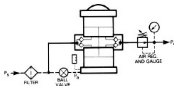
SEMI-STANDARD AIR CONTROLS — AAD-2 Only
