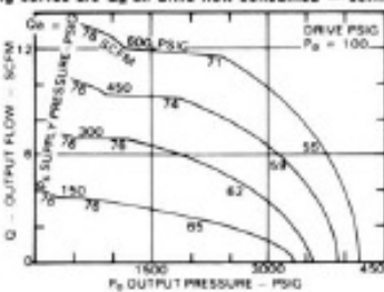
MODEL AAT-15/30 Two Stage (Intermediate numbers along curves are Qa air drive flow consumed — scfm.)
